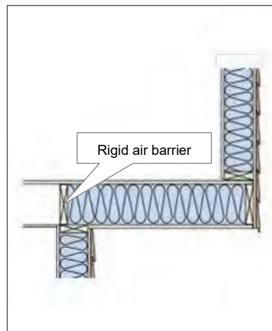
Cantilever Floor Area
