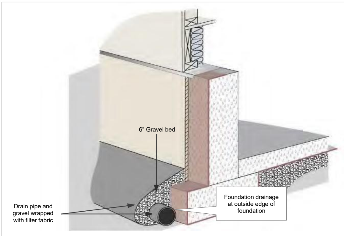
Foundation Drainage System Outside Perimeter Edge of Crawlspace Wall Footing
