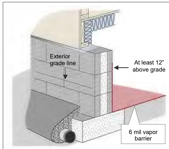
Vapor Barrier Installed in Crawlspace
