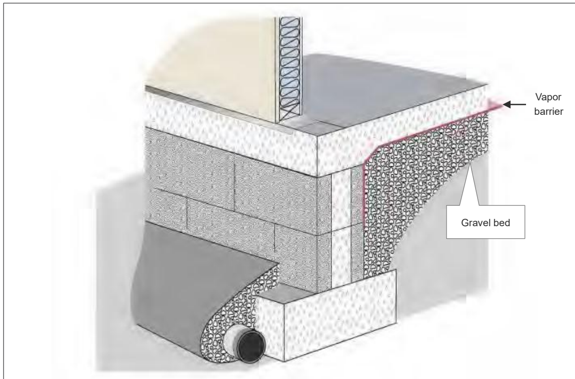
Gravel Bed Beneath Vapor Barrier
