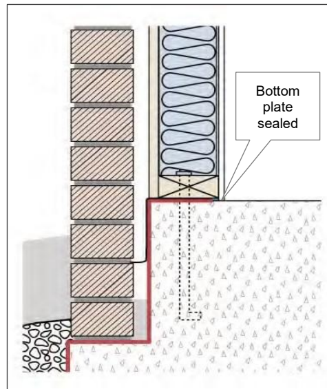
Bottom Plate Sealed to Slab
