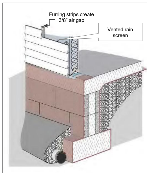
Vented Rain Screen - Cladding
