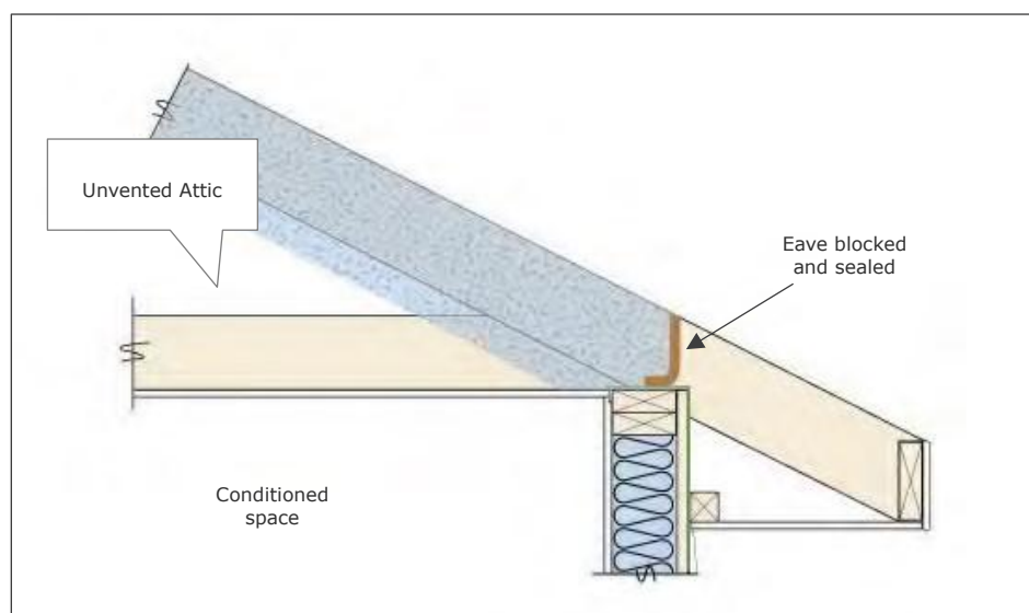
Example: Insulation Applied Under Roof Deck
