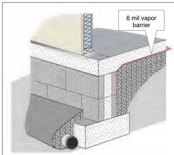
Vapor Barrier Installed Beneath Slab
