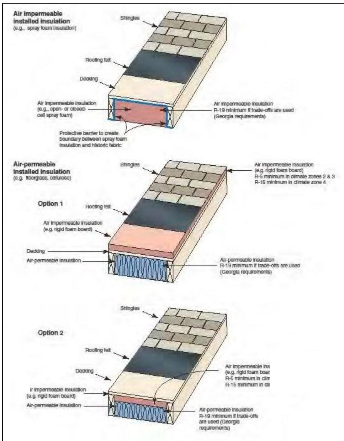
Unvented Attic - Roofline Installed Insulation Options (refer to 2009 IRC)
