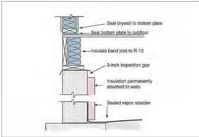
Closed Crawlspace Wall Details
