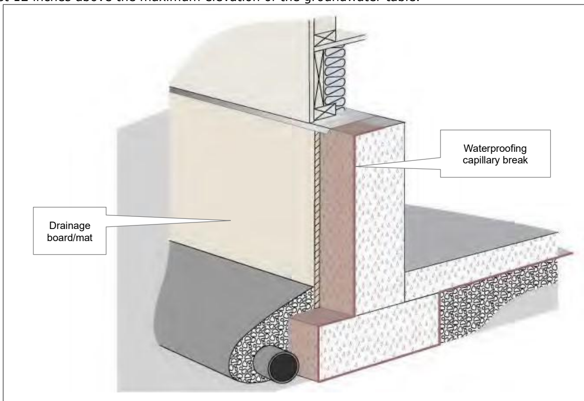
Drainage Plane Applied At Below Grade Wall
