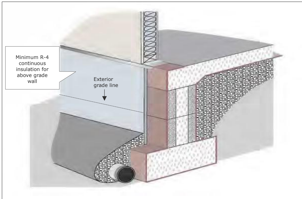
Insulation at Foundation Wall
