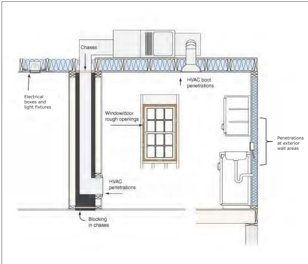
Typical Air Barrier Penetrations at Building Thermal Envelope
