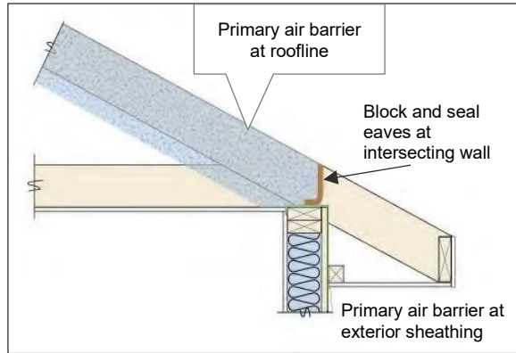
Continuous Air Barrier - Unvented Attic
