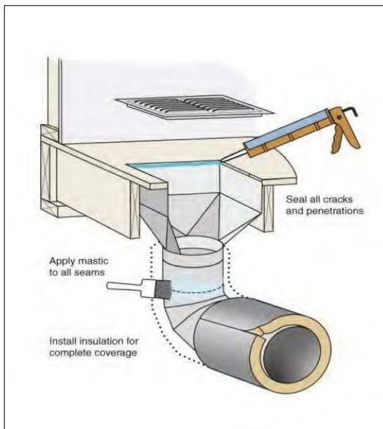
Duct Sealing Locations at Branch and Boot
