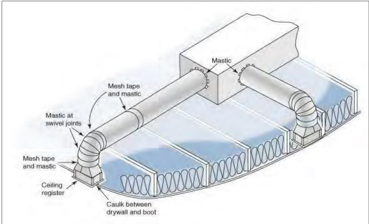
Duct Sealing Locations at Trunk and Branches
