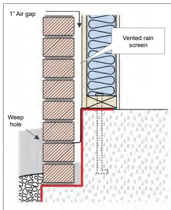
Vented Rain Screen – Masonry Veneer
