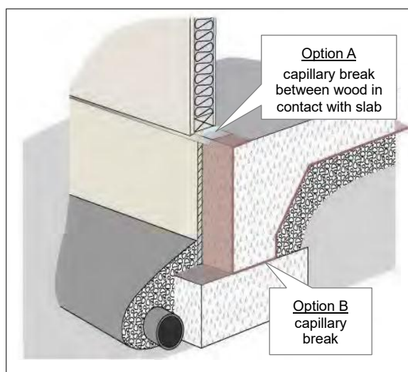
Capillary Break Between Footing and Slab
