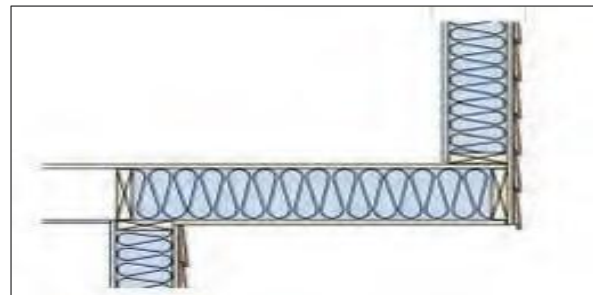
Cantilever Floor Area
