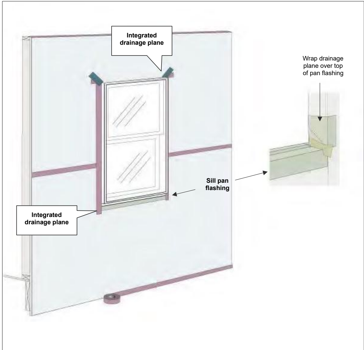
Integrated Flashing at Window Penetration
