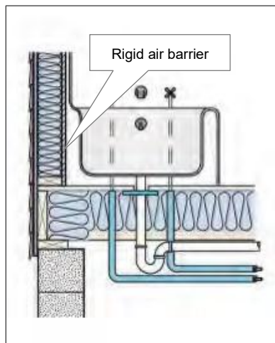
Exterior Wall at Tub Area
