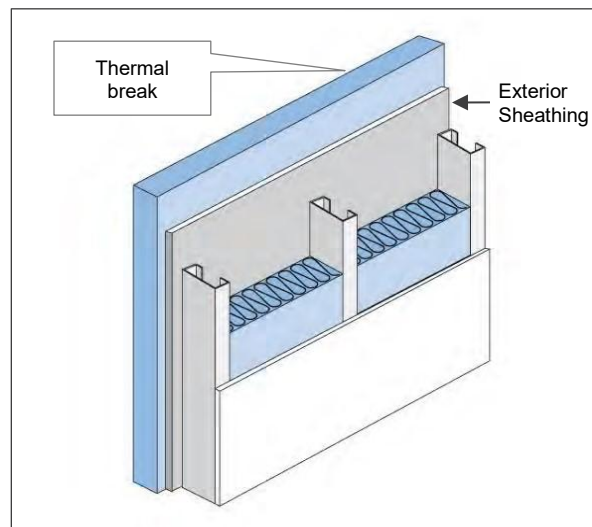
Steel Stud Framed Wall Section
