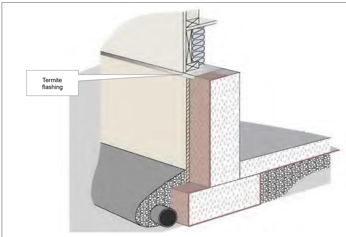
Termite Shield Between Wood Framing and Foundation Stem Wall
