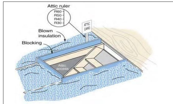
Insulated Attic
