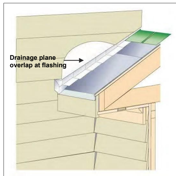
Flashing at Roof – to – Wall Intersection
