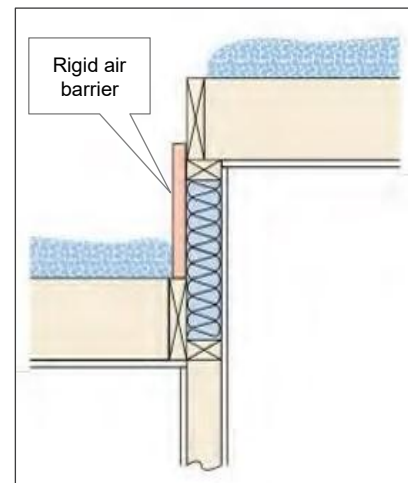
Kneewall Area at Raised Ceiling
