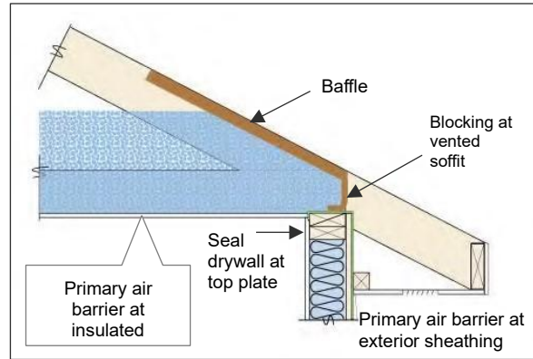
Continuous Air Barrier - Vented Attic
