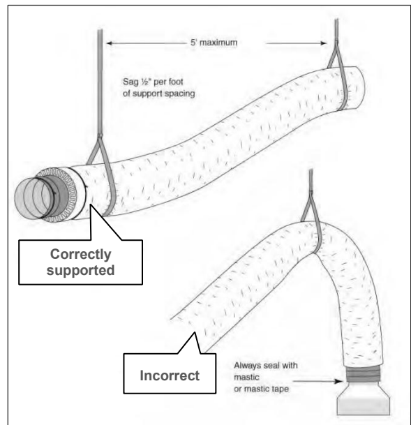
Flex Duct Support
