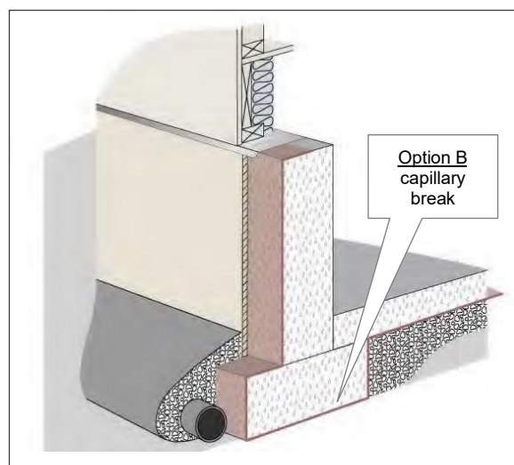
Capillary Break Beneath Footing
