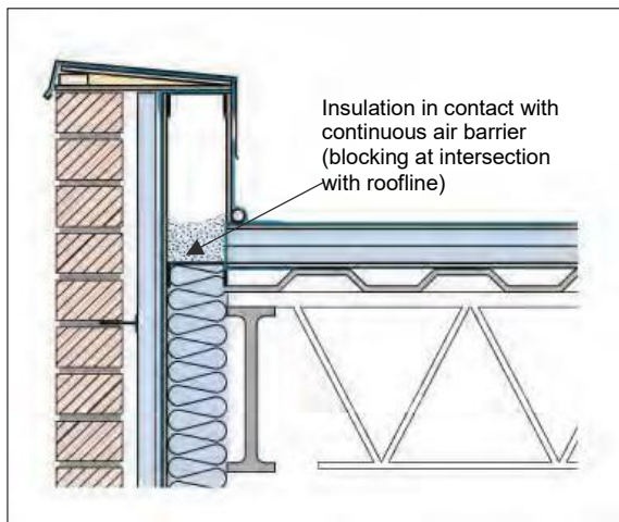
Parapet: Example 1
