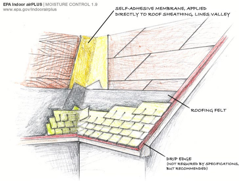
MEMBRANE PROTECTION OF ROOF VALLEY
