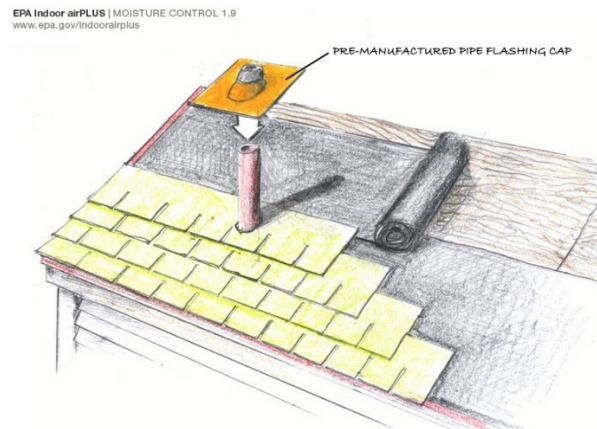
SHINGLES PLACED OVER MEMBRANE AND FELT
