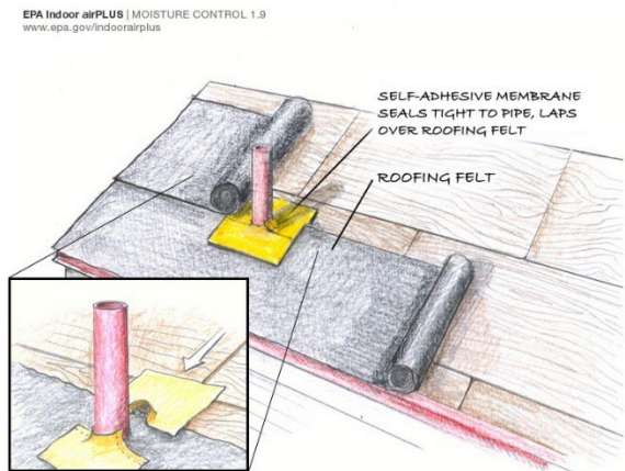
PLUMBING VENT STACK - 'PEEL AND STICK' MEMBRANE
